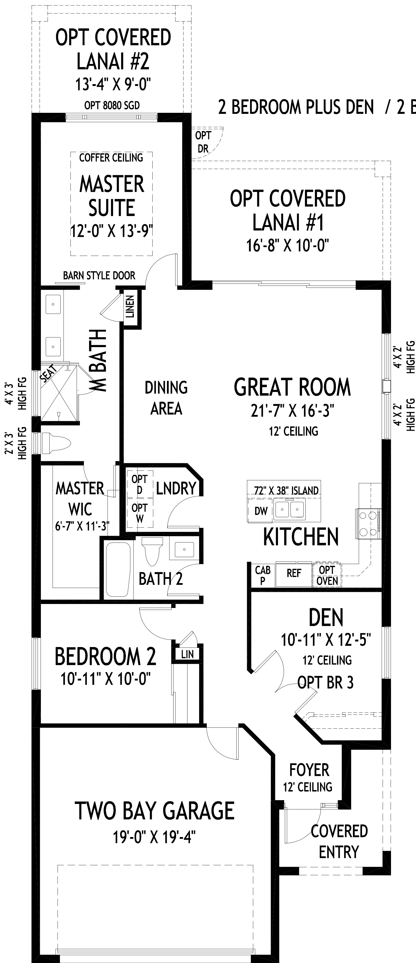
FLOOR PLAN
